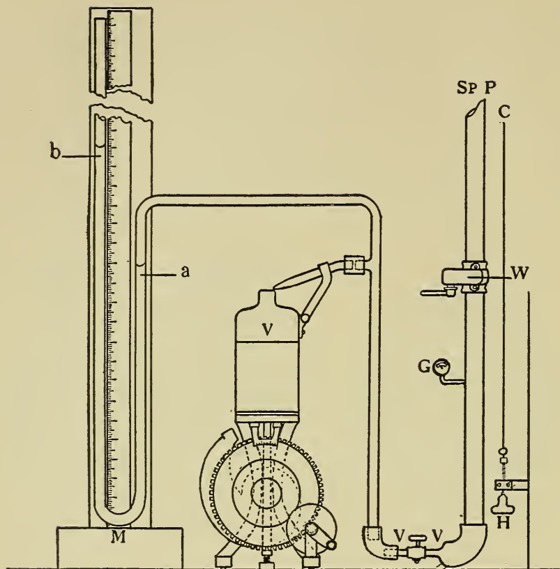
FIG. 10. METHOD OF USING AIR SUPPLY
